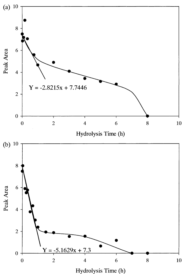
Fig. 2. Reduction rate of \nu\text{C-N} peak at 1275\text{ cm}^{-1} of the mixture containing 1\text{SiO}_2:0.5\text{Al}_2\text{O}_3:0.096\text{Na}_2\text{O}:63\text{H}_2\text{O} in (a) NaCl/H 2 O.
