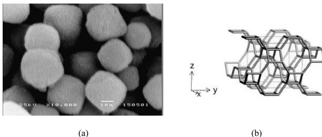
Fig. 8. SEM micrographs of (a) Na-PI zeolite (GIS) and (b) the unite cell structure.
