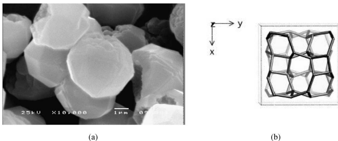
Fig. 6. SEM micrographs of (a) analcime zeolite (ANA) and (b) the unit cell structure.
