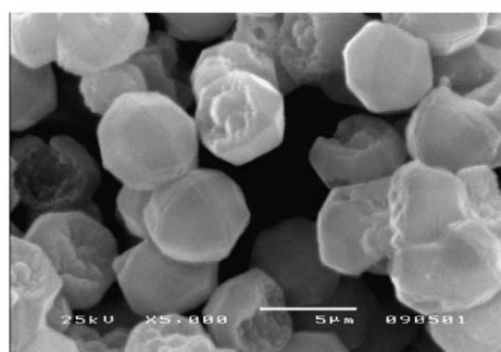
Fig. 11. SEM micrographs of aluminosilicate synthesized from 1\text{SiO}_2:0.25\text{Al}_2\text{O}_3:3\text{Na}_2\text{O}:3\text{Na}_2\text{O}:410\text{H}_2\text{O} at 130 °C/ x h ( x = 1-9 h).
