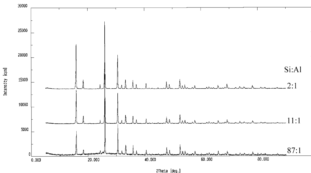
Fig. 5. Effect of Si:Al ratio (2:1–87:1) on microwave heated aluminosilicate synthesized from 1\text{SiO}_2:x\text{Al}_2\text{O}_3:3\text{Na}_2\text{O}:410\text{H}_2\text{O} ( x=0.01149-0.25 ) at 150^\circ\text{C}/15\text{ h} .
