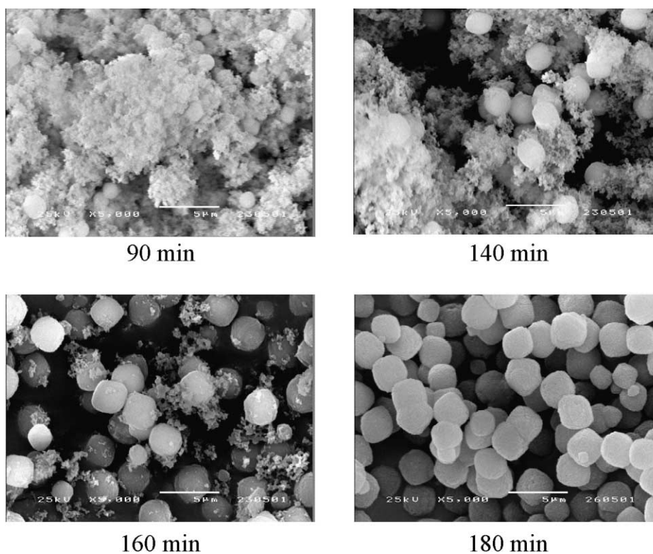
Fig. 13. SEM micrographs of aluminosilicate synthesized from 1\text{SiO}_2:0.25\text{Al}_2\text{O}_3:3\text{Na}_2\text{O}:410\text{H}_2\text{O} at 110^\circ\text{C}/x\text{ h} ( x=1.5\text{--}4\text{ h} ).
