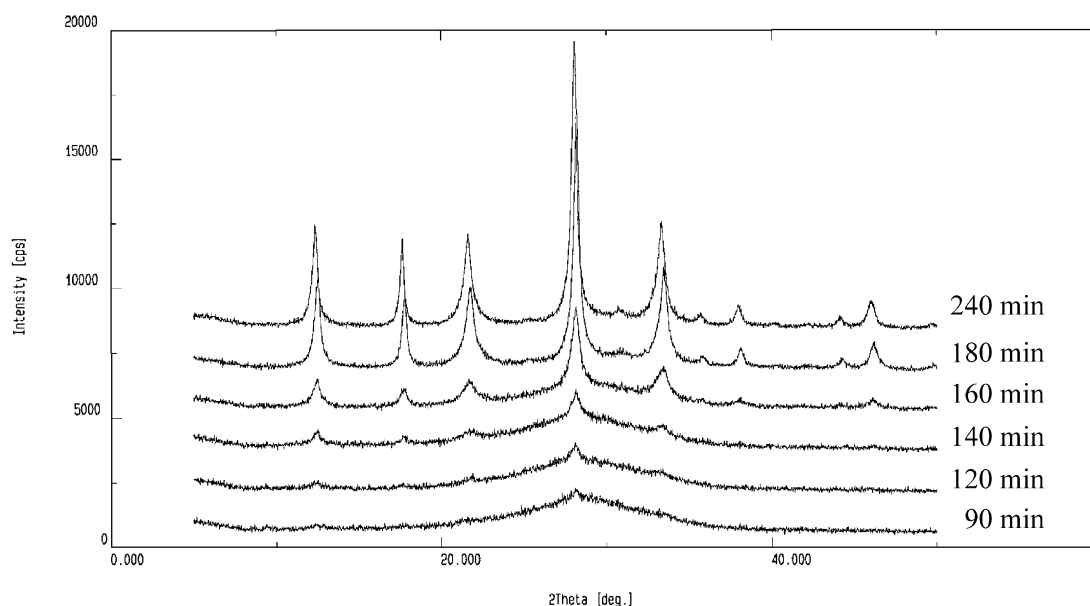
Fig. 12. Effect of microwave heating time on aluminosilicate synthesized at 1\text{SiO}_2:0.25\text{Al}_2\text{O}_3:3\text{Na}_2\text{O}:410\text{H}_2\text{O} and 110^\circ\text{C}/x\text{ h} ( x=1.5\text{--}4\text{ h} ).
