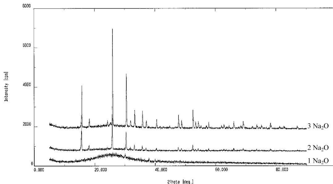
Fig. 4. Effect of NaOH concentration of microwave heated aluminosilicate synthesized from 1\text{SiO}_2:0.0115\text{Al}_2\text{O}_3:x\text{Na}_2\text{O}:410\text{H}_2\text{O} ( \text{Si}:\text{Al}=87:1, x=1-3 ) at 150^\circ\text{C}/15\text{ h} .
