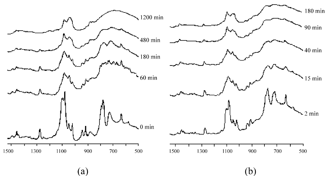
Fig. 1. Hydrolysis behavior of alumatrane and silatrane mixture at the ration of 1SiO 2 :0.5Al 2 O 3 :0.096Na 2 O:63H 2 O in (a) NaCl/H 2 O system and (b) NaOH/H 2 O system.
