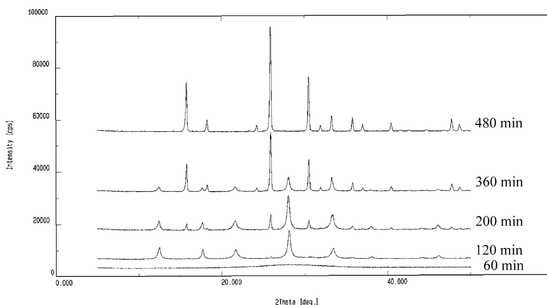
Fig. 9. Effect of microwave heating time on aluminosilicate synthesized from 1\text{SiO}_2:0.25\text{Al}_2\text{O}_3:3\text{Na}_2\text{O}:410\text{H}_2\text{O} at 130 °C/ x h ( x=1-9 h).
