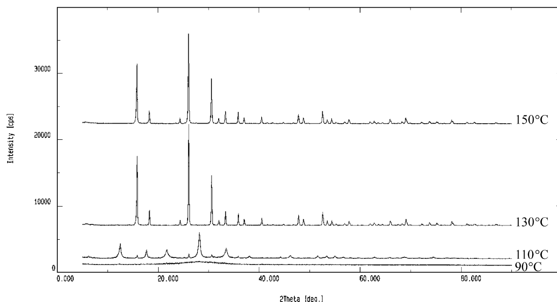
Fig. 7. Effect of microwave heating temperature on aluminosilicate synthesized from 1\text{SiO}_2:0.091\text{Al}_2\text{O}_3:3\text{Na}_2\text{O}:410\text{H}_2\text{O} at x^\circ\text{C}/15\text{ h} ( x=90\text{--}150^\circ\text{C} ).
