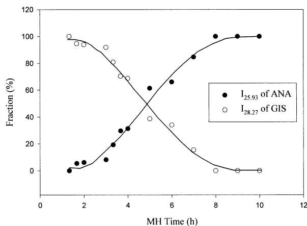
Fig. 10. Fraction of GIS and ANA calculated from XRD area under the peak at 25.93 (2θ) for ANA and 28.27 (2θ) for GIS.
