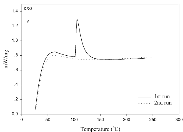
Fig. 3. Thermal property of gel transference to aluminosilicate using high pressure DSC cell at heating rate of 10\text{ }^\circ\text{C/min} and 1\text{SiO}_2:0.5\text{Al}_2\text{O}_3:0.7\text{Na}_2\text{O}:410\text{H}_2\text{O} .
