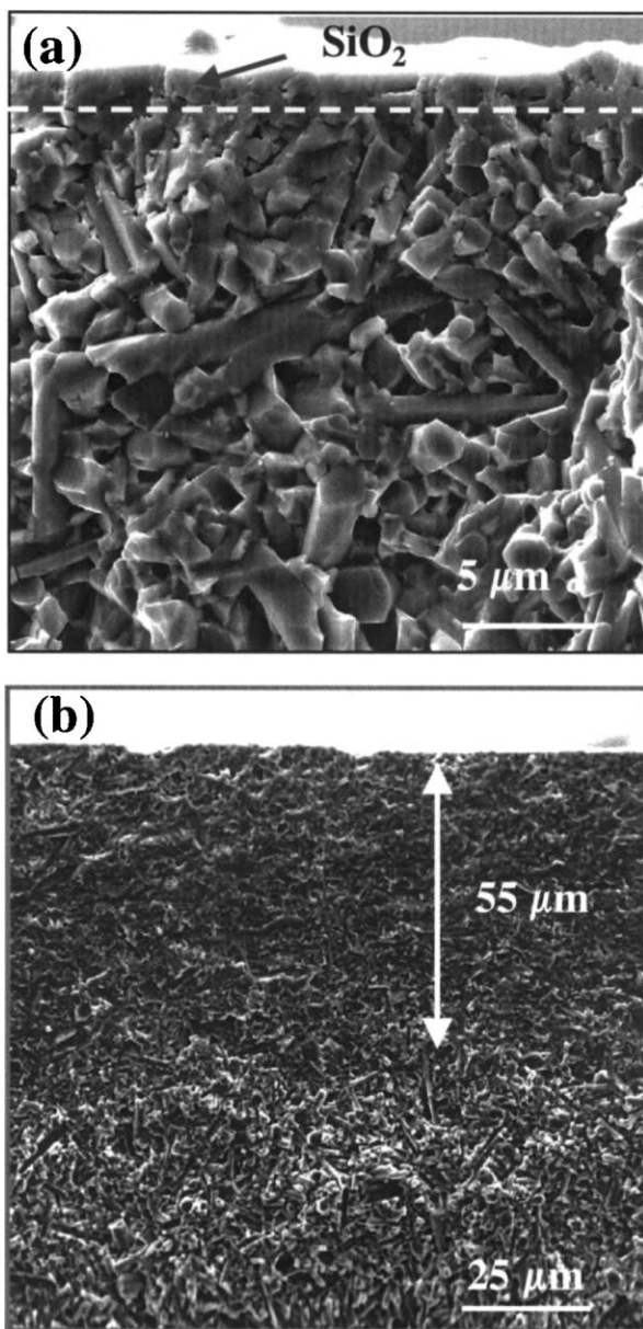
Fig. 9. Fracture surface of disk samples from airfoil surface of (a) as-received vane and (b) vane after 525 h engine test.
