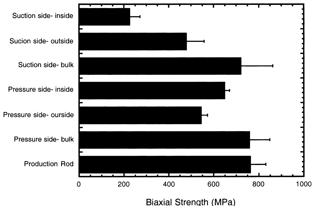
Fig. 11. Strength summary for samples extracted from the as-manufactured FT8 air-cooled SN282 silicon nitride vane.
