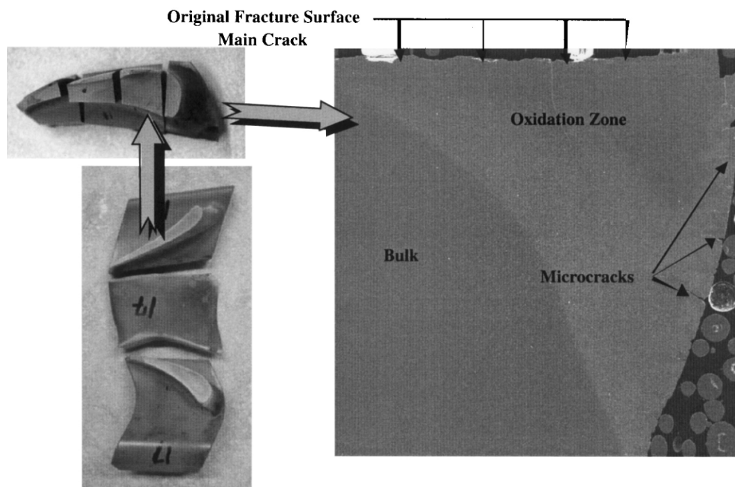
Fig. 3. Cross-section of failed nozzle showing damage zone evolution in the vicinity of the primary fracture surface. The light-colored zone was found to exhibit a higher oxygen content compared to the bulk material.
