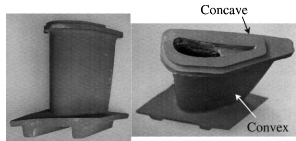
Fig. 10. As manufactured FT8 air-cooled SN282 silicon nitride vane.
