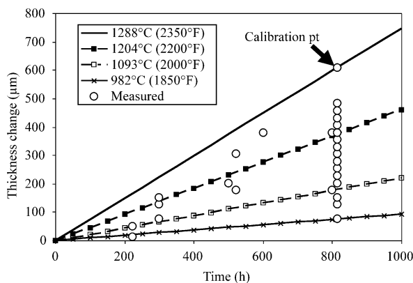
Fig. 5. Measurement of recession of the silicon nitride vanes at the mid-span of the trailing edge (open circles). The solid lines in this figure represent predictions based upon a model described in the Introduction.
