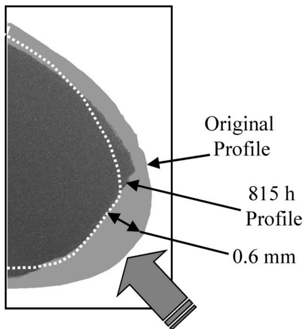
Fig. 6. Profiles of leading edge (midspan) before testing and after 815 h. The large black arrow indicates gas flow direction.
