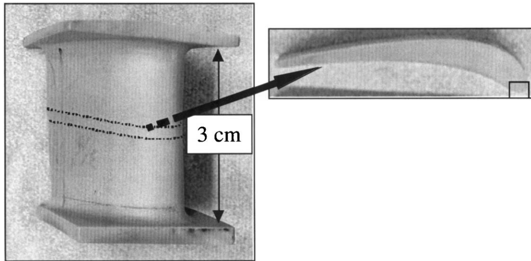
Fig. 4. Sectioning of vanes required for SEM of cross-sections.
