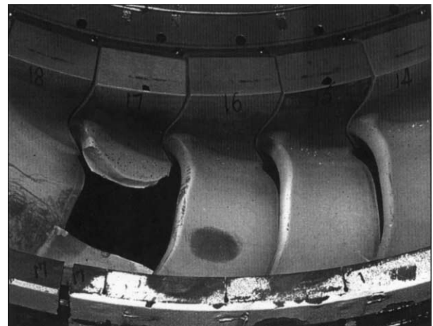
Fig. 2. Nozzle assembly after 68 h test showing failed nozzle.
