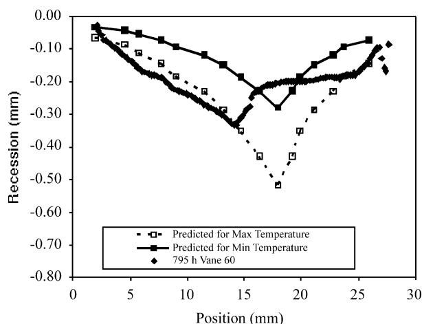
Fig. 7. Comparison of measured and predicted recession along the trailing edge.
