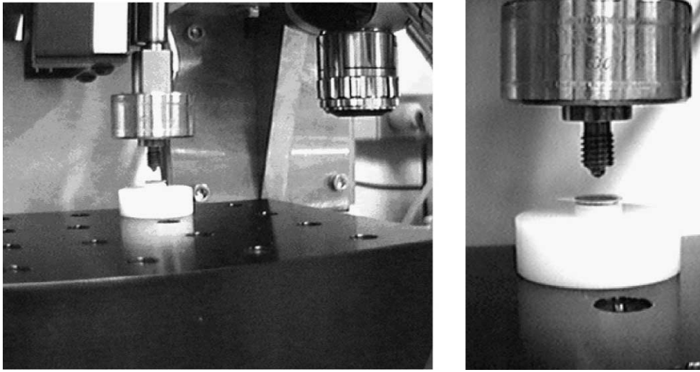
Fig. 1. Biaxial test fixture and specimen.
