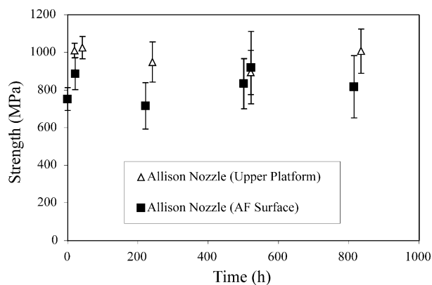
Fig. 8. Biaxial flexure strength data of AS800 vanes versus engine exposure time.
