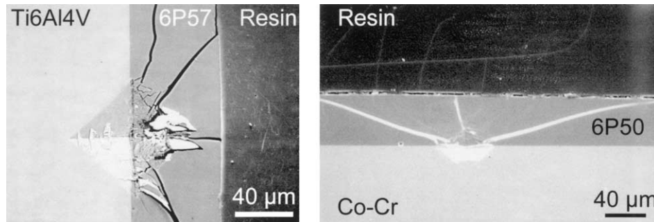
Fig. 5. Vickers indentations at the glass 6P57/Ti6Al4V (1.2 kg) and 6P50/Co-Cr (0.6 kg) interfaces performed in ambient air. The cracks were driven towards the glass and the coating did not delaminate qualitatively indicating good glass-metal adhesion.
