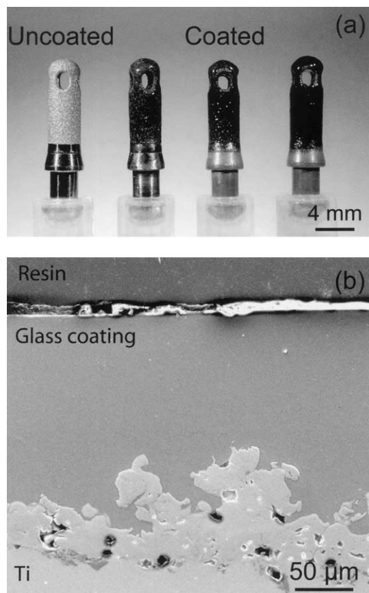
Fig. 11. Coated titanium internal hexagonal cylinder implants (a) and corresponding SEM of a polished cross section (b). During firing the glass has flown establishing good contact with the rough implant surface.
