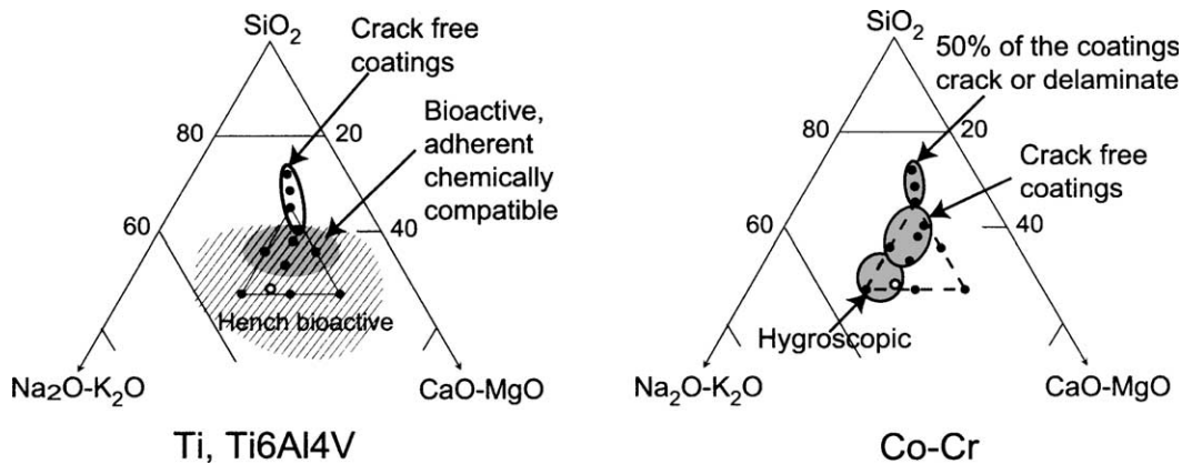
Fig. 3. Compositional triangles showing the adequate composition ranges to coat Co–Cr and Ti-based alloys. All glasses have a constant 6 wt.% \text{P}_2\text{O}_5 content.
