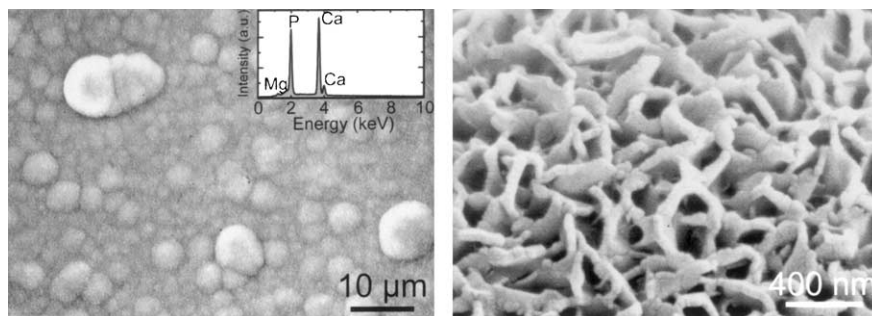
Fig. 9. SEM micrograph and associated EDS analysis of apatite crystals precipitated on a 6P57 coating after 30 days in SBF.
