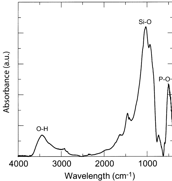
Fig. 2. FTIR analysis of Bioglass ® powder stored for one month in air. The presence of a strong O–H hydration bands is clearly visible.
