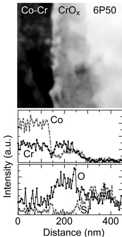
Fig. 8. TEM image and associated line analysis of the interface between glass 6P50 and a Co–Cr alloy after firing at 750°C for 30 sec.
