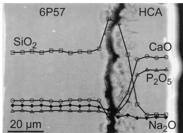
Fig. 10. Elemental cross section analysis (SEM-EDS) of a 6P57 coating after 2 months in SBF. A \sim 20 \mu\text{m} thick apatite layer is visible on the 6P57 coating surface growing on a Si-rich region.
