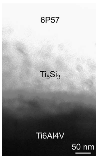
Fig. 7. TEM image of the cross section of a 6P57 glass coating on Ti6Al4V annealed at 800 °C for 30 sec.
