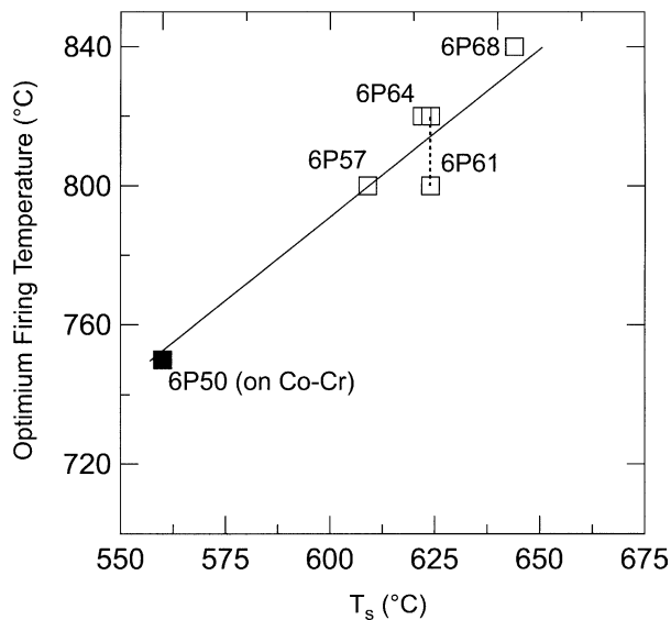
Fig. 6. Relationship between the optimum firing temperature and the softening point of the glasses.
