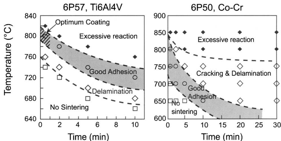
Fig. 4. Influence of firing time and temperature on the adhesion of coatings manufactured with glass 6P57 on Ti6Al4V and glass 6P50 on Co–Cr.
