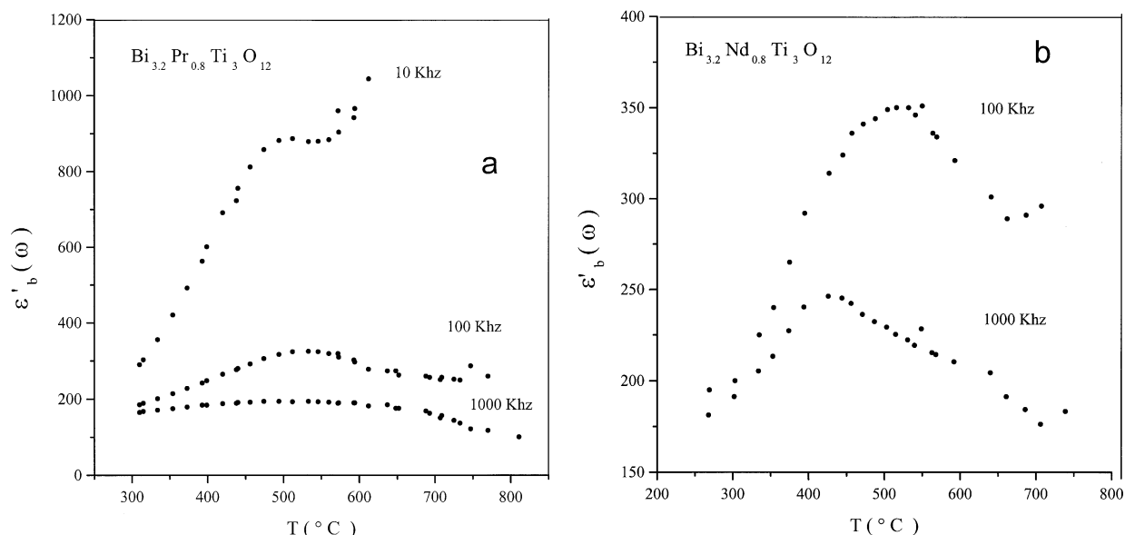
Fig. 9. Real part \varepsilon'(\omega) of the permittivity versus temperature for selected frequencies (a) \text{Bi}_{3.2}\text{Pr}_{0.8}\text{Ti}_3\text{O}_{12} , (b) \text{Bi}_{3.2}\text{Nd}_{0.8}\text{Ti}_3\text{O}_{12} .
