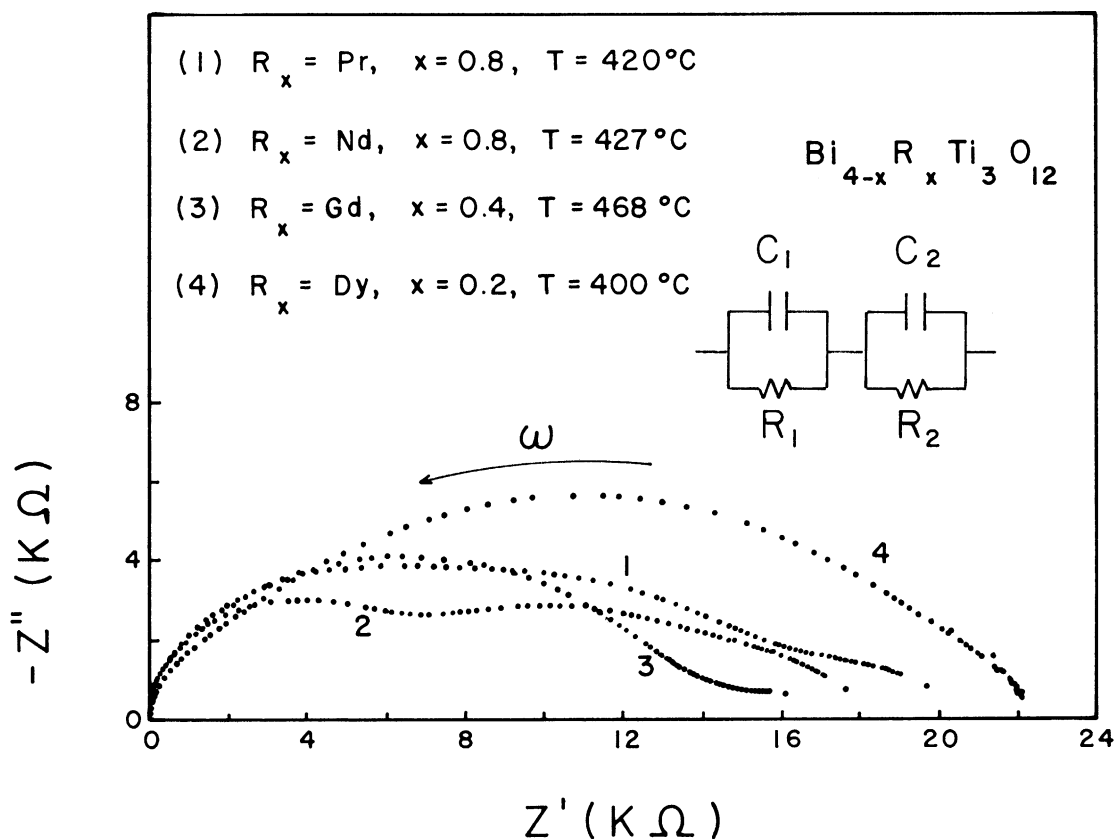
Fig. 4. Typical impedance curves for \text{Bi}_{4-x}\text{R}_x\text{Ti}_3\text{O}_{12} ( \text{R}_x = \text{Pr, Nd, Gd and Dy} ). Curves were chosen for selected temperatures. The equivalent circuit is shown as well.
