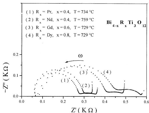
Fig. 10. Impedance curves at temperatures above 550^\circ\text{C} for R_x = \text{Pr} , \text{Nd} , \text{Gd} , \text{Dy} . Is shown well-formed spikes.
