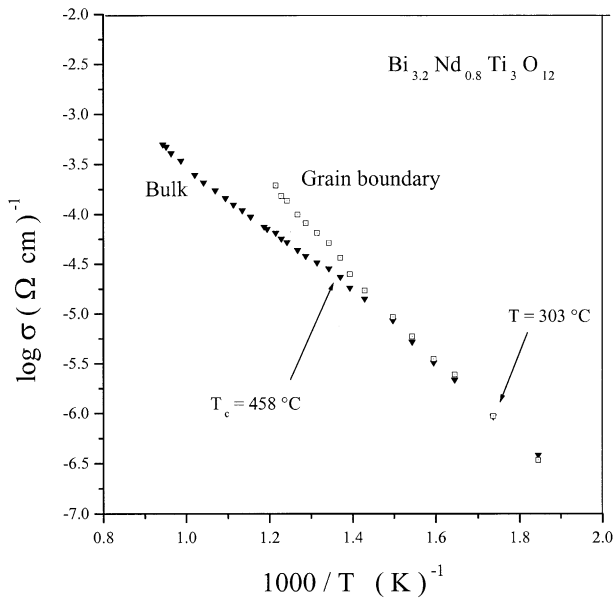
Fig. 7. Typical variation of \sigma_b and \sigma_{gb} with temperature for \text{Bi}_{3.2}\text{Nd}_{0.8}\text{Ti}_3\text{O}_{12} . Two temperatures are shown: T_c = 458 °C the ferro-paraelectric transition temperature of the compound; 303 °C points out temperature for which, Arrhenius plot for bulk and grain boundary intersect.
