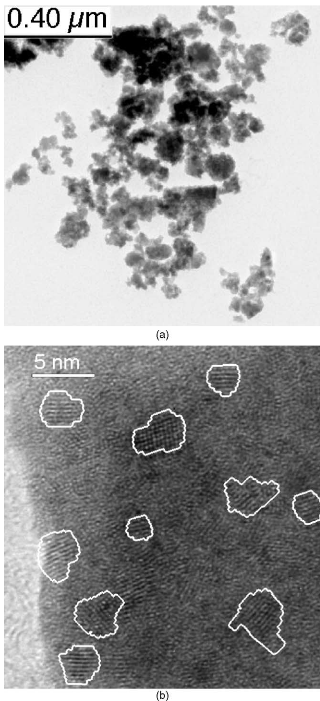
Fig. 3. HR-TEM micrographs of the sol-prepared powder of \text{BaSn(OH)}_6 : (a) diffraction contrast imaging, (b) structure imaging. \text{BaSn(OH)}_6 was hydrothermally synthesised from the \text{SnO}_2 \cdot x\text{H}_2\text{O} sol and \text{Ba(OH)}_2 at 250^\circ\text{C} for 6 h.
