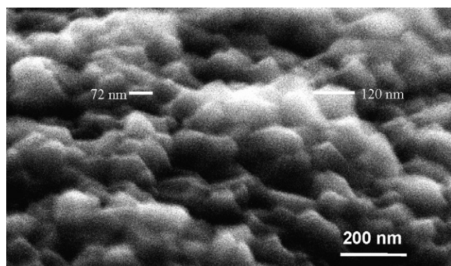
Fig. 6. SEM image of a dense ceramic with average grain size 75 nm.
