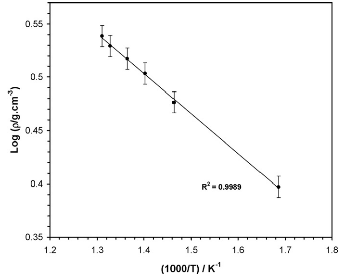
Fig. 3. Arrhenius plot of density values up to 490^\circ\text{C} .
