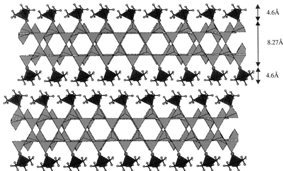
Fig. 6. Proposed structure of the lamellar silica phase after silylating. Light grey tetrahedra constitute \text{SiO}_2 layers with tridymite crystal structure, dark grey tetrahedra represent the grafted TMS groups.
