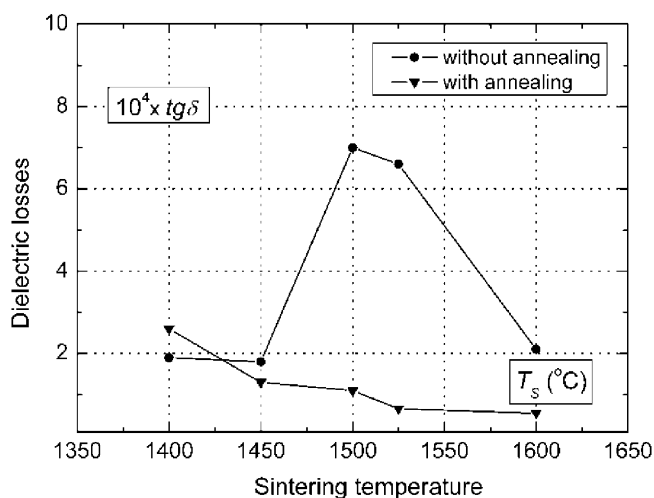
Fig. 7. Modification of dielectric losses curve vs. sintering temperature for BZT ceramics without and with annealing treatment at 1400 °C/10 h.
