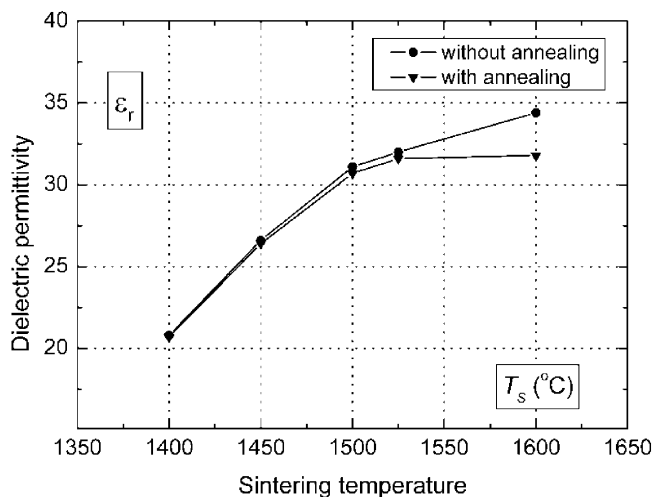
Fig. 8. Modification of dielectric permittivity curve vs. sintering temperature for BZT ceramics without and with annealing treatment at 1400 °C/10 h.
