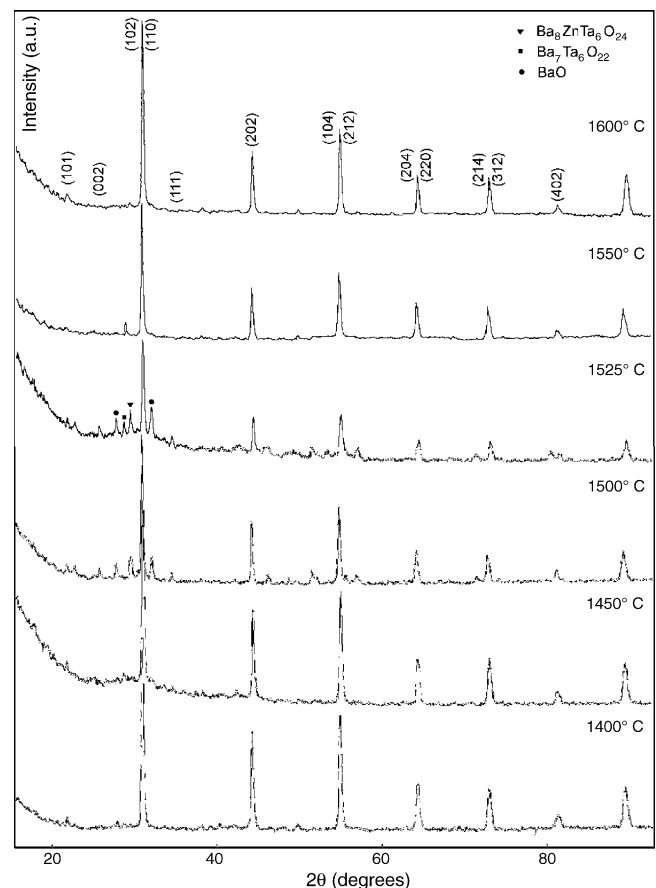
Fig. 1. XRD patterns of \text{Ba}(\text{Zn}_{1/3}\text{Ta}_{2/3})\text{O}_3 system vs. sintering temperature.
