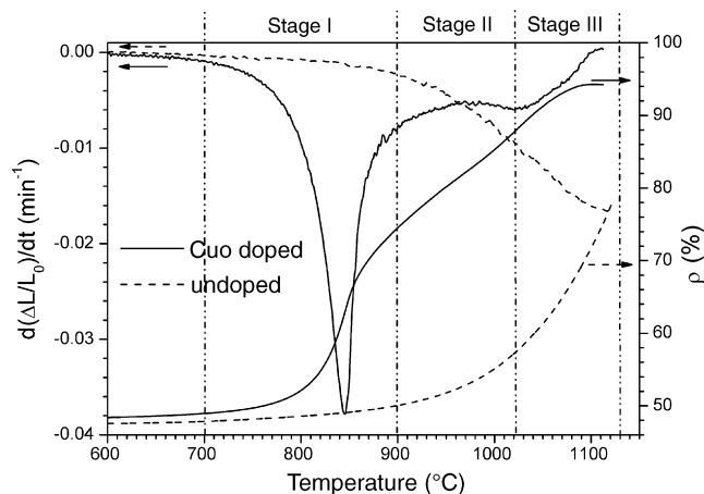
Fig. 1. Density and linear shrinkage rate as functions of temperature during heating. Solid lines are of 8 mol% CuO doped 3Y-TZP nano-powder composite; dashed lines are of undoped 3Y-TZP nano-powder compact.
