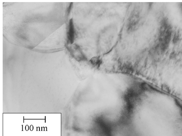
Fig. 3. TEM image of 8 mol% CuO doped 3Y-TZP nano-powder composite sintered at 1130 °C for 1 h in an oxygen flow.
