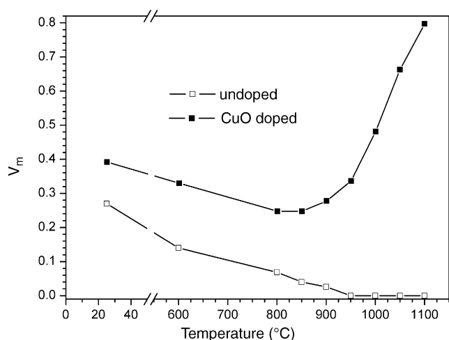
Fig. 4. Volume fraction of monoclinic zirconia as a function of temperature during heating. Solid square symbols are of 8 mol% CuO doped 3Y-TZP nano-powder composite; open square symbols are of undoped 3Y-TZP.
