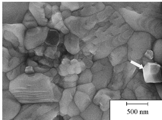
Fig. 2. Cross-section SEM image of 8 mol% CuO doped 3Y-TZP nano-powder composite sintered at 1130 °C for 1 h in an oxygen flow.
