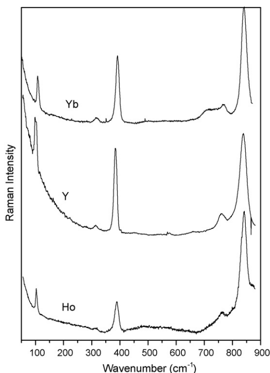
Fig. 3. Micro-Raman spectra of the \text{Ba}(\text{RE}_{1/2}\text{Ta}_{1/2})\text{O}_3 ceramics [RE = Yb, Y, and Ho] with cubic symmetry.
