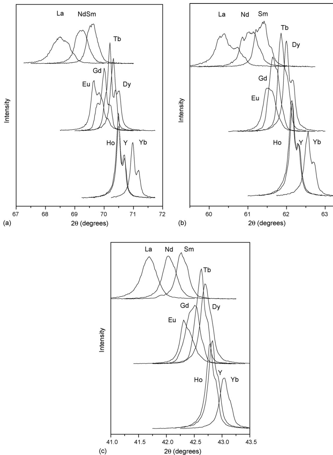
Fig. 2. X-ray powder diffraction for the Ba(RE 1/2 Ta 1/2 )O 3 ceramics. (a) Detail for the range 67–72° 2θ, showing the splitting of the cubic (6 2 0) peak. Doubling of the reflections for Yb, Y and Ho accounts for K α1 (1.54051 Å) and K α2 (1.54433 Å) lines. (b) Detail for the range 59.5–63.3° 2θ, around the cubic (4 4 0) peak. (c) Detail for the range 41.0–43.5° 2θ, around the cubic (4 0 0) peak.
